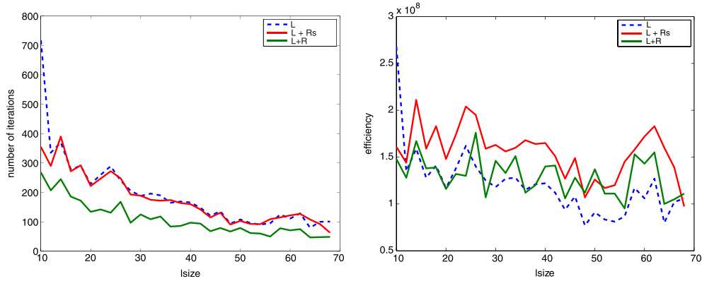
FIGURE 2 Iteration counts (left) and efficiency (right) for problem Schenk_IBMNA/c-56 with lsize = rsiz e varying
