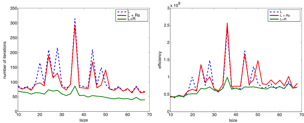
FIGURE 3 Iteration counts (left) and efficiency (right) for problem PARSEC/CO with lsize = rsiz e varying
