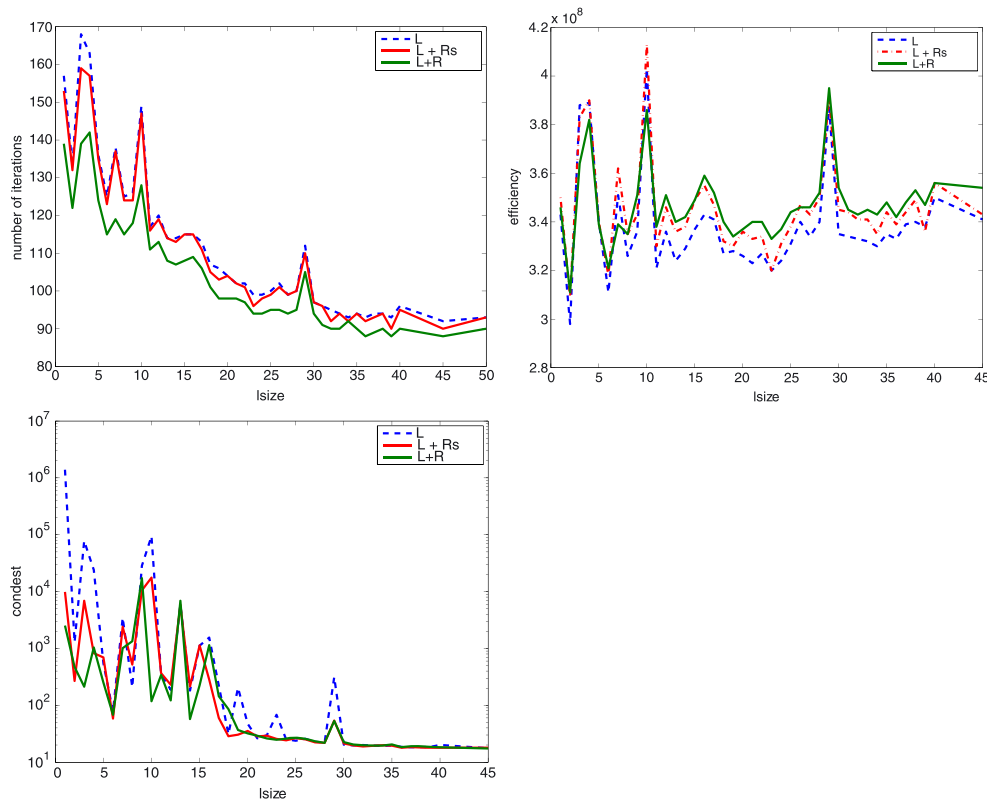
FIGURE 1 Iteration counts (top left), efficiency (top right), and condest (bottom left) for problem PARSEC/Ga3As3H12 with rsize = 5 and lsize varying
