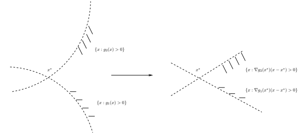
FIG. 2.6. Two active inequality constraints intersect properly
