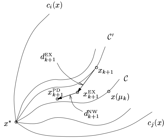
Figure 5.1: The above picture simplifies the situation as the x -space only is considered. The infeasible region is the “outer” part of the picture. Constraints i and j are active at the local constrained minimizer x^* . The exact solution of the current barrier subproblem, x(\mu_k) , lies exactly on the primal-dual central path \mathcal{C} . The second path \mathcal{C}' that is pictured is defined implicitly by \Psi(w; \mu) = \Psi(w_{k+1}; \mu_k) as in equation (5.93). The two outermost paths represent the neighborhood of \mathcal{C} defined by the forcing functions \epsilon^C(\mu) and \epsilon^D(\mu) . The extrapolated step d_{k+1}^{\text{EX}} taken from w_{k+1} leaves the path \mathcal{C}' tangentially and leads to w_{k+1}^{\text{EX}} . To that step is added the Newton step d_{k+1}^{\text{NW}} that would have been taken from w_{k+1} , as represented on the picture. The step d_{k+1}^{\text{EX}} + d_{k+1}^{\text{NW}} is the step leading to w_{k+1}^{\text{PD}} as given by (5.89).
