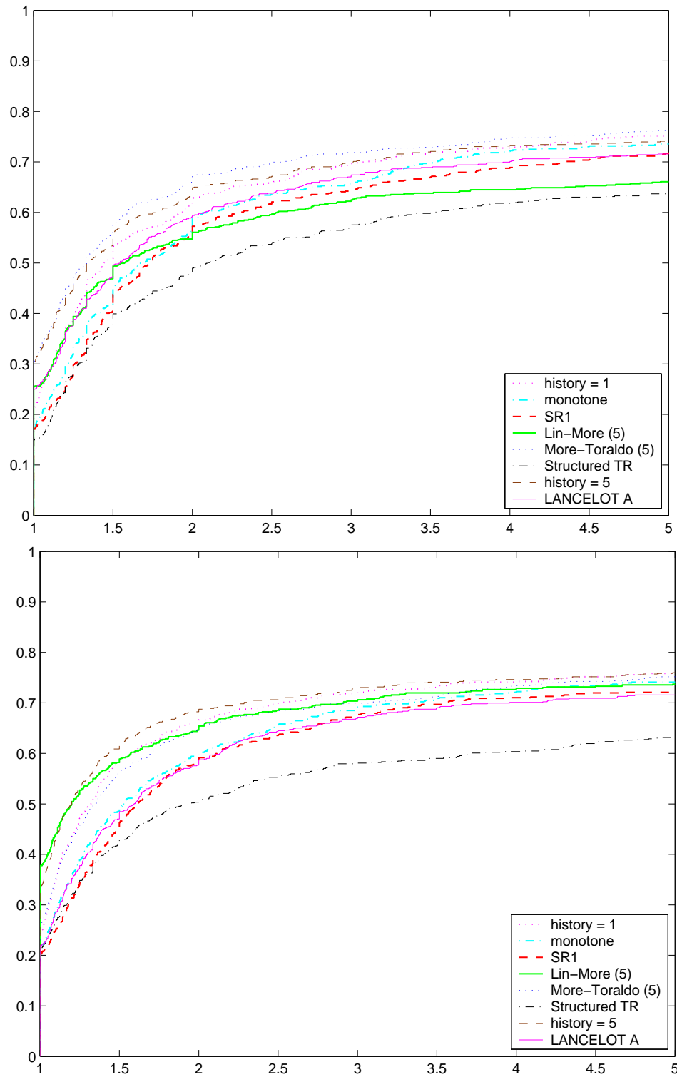
Figure 2.1: Performance profile for LANCELOT options: CPU times (top) and number of function evaluations (bottom). The horizontal axis gives the argument \sigma , while the vertical axis records p_i(\sigma) for each of the competing options, i .
