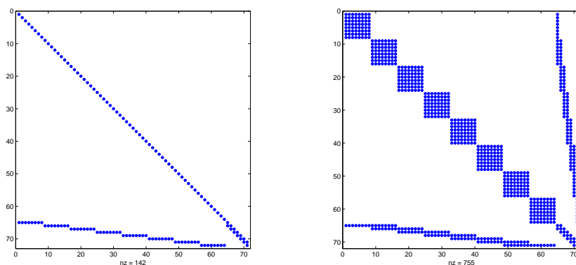
FIG. 2.1. Structure of \hat{A} (left) and \hat{C} (right) for the matrix A with a single dense row and A_s diagonal with n = 64 and the dense row stretched into 8 parts.
