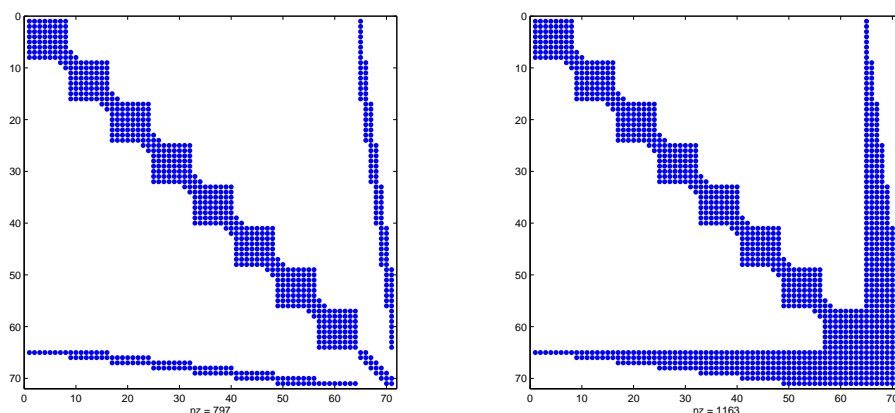
FIG. 2.3. Structure of \hat{C} and its Cholesky factor for the matrix A with A_s tridiagonal and a single dense row that is split into 8 parts ( n = 64 ).
