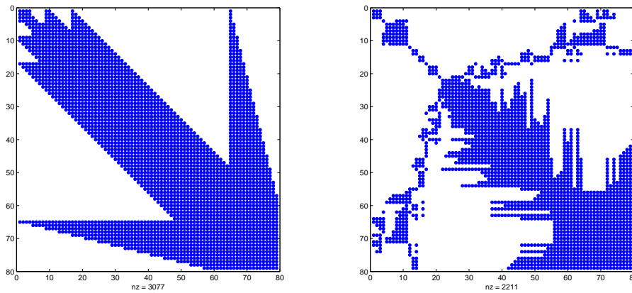
FIG. 2.6. Structure of the Cholesky factor of the stretched normal matrix with no reordering (left) and AMD ordering (right). A_s has the structure of the five-point two-dimensional discrete Laplacian matrix; one dense row is appended and split into 8 parts ( n = 64 ).
