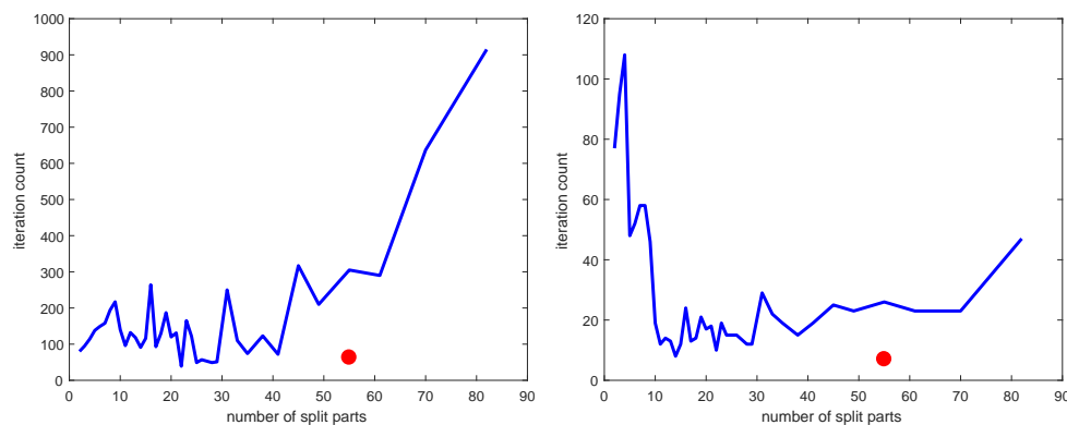
FIG. 4.9. Comparison of iteration counts for standard and sparse stretching for problem LP_AGG with one dense row appended. The dot is for sparse stretching. Here lsize = 25 (left) and lsize = 50 (right).
