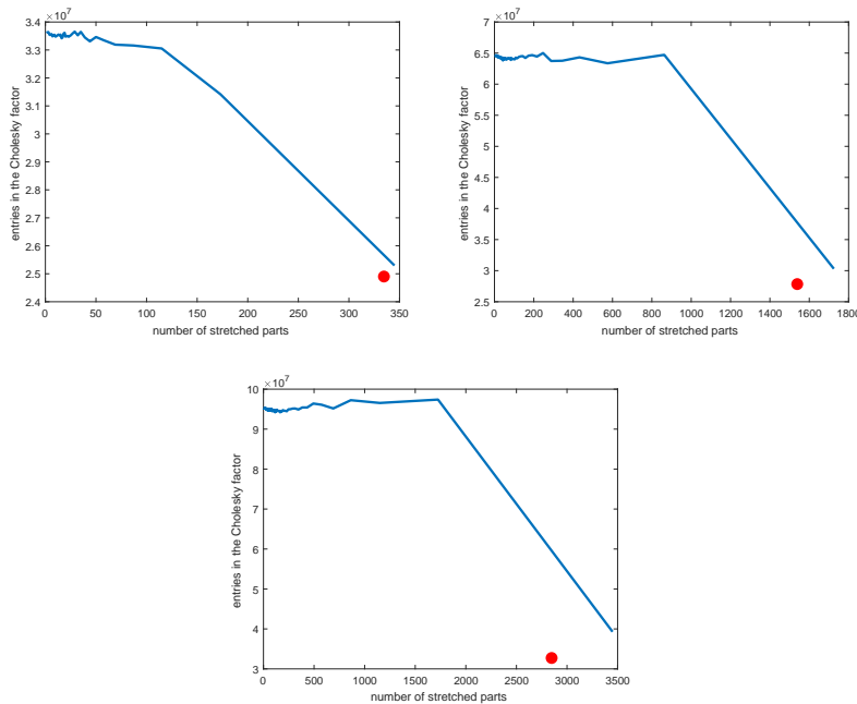
FIG. 4.7. Problem WORLD with one appended row of density \rho = 0.01, 0.05 , and 0.1 . In each case, the number of entries in the Cholesky factor of the stretched normal matrix is reported. The curves correspond to the number of entries varying with the number of parts into which the dense row is stretched (standard stretching); the dot is for sparse stretching with the number of stretched parts determined by Algorithm 3.1.
