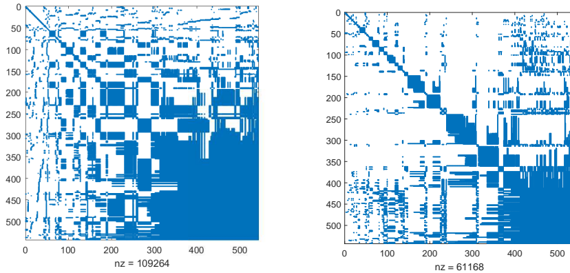
FIG. 4.5. For problem LP_AGG with one dense row appended, the sparsity pattern of the Cholesky factor of the AMD reordered stretched normal matrix for standard stretching (left) and sparse stretching (right) with the number of stretched parts determined by Algorithm 3.1.
