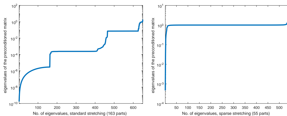
FIG. 4.10. Spectrum of the preconditioned stretched normal matrix. Standard stretching with k = 163 (left) and sparse stretching ( k = 55 ) (right). Here lsize = 25 .
