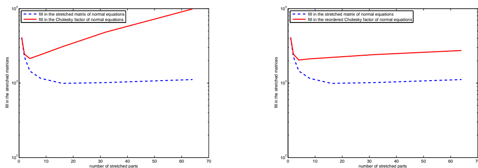
FIG. 2.7. Number of nonzeros in the Cholesky factor of \hat{C} with no reordering (left) and with AMD ordering (right) as the number of stretched parts increases. A_s has the structure of the five-point two-dimensional discrete Laplacian matrix, and one dense row is appended ( n = 64 ).
