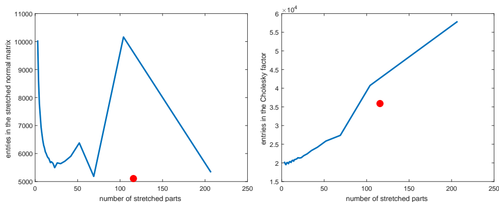
FIG. 4.1. Comparison of the entries in the stretched normal matrix (left) and its Cholesky factor (right) for problem WM1 with one dense row appended. The curve corresponds to the number of entries varying with the number of parts into which the dense row is stretched (standard stretching); the dot is for sparse stretching with the number of stretched parts determined by Algorithm 3.1 ( k = 116 ).
