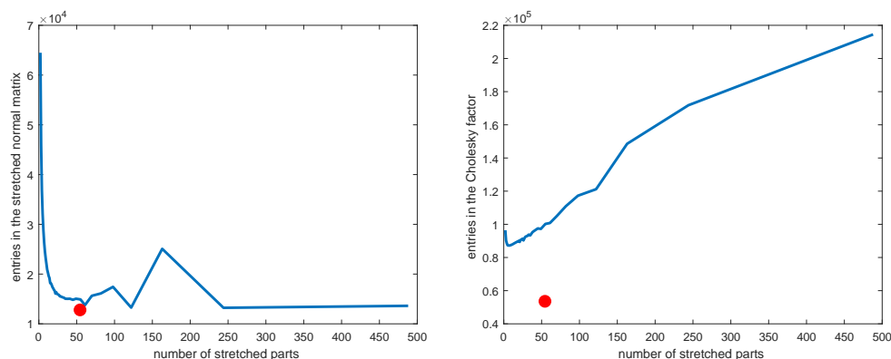
FIG. 4.2. Comparison of the entries in the stretched normal matrix (left) and its Cholesky factor (right) for problem LP_AGG with one dense row appended. The curve corresponds to the number of entries varying with the number of parts into which the dense row is stretched (standard stretching); the dot is for sparse stretching with the number of stretched parts determined by Algorithm 3.1 ( k = 55 ).
