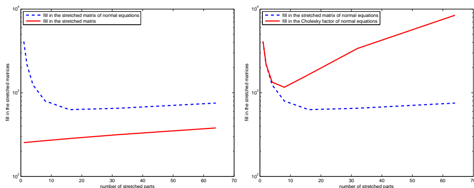
FIG. 2.4. Number of nonzeros in \hat{A} and \hat{C} (left) and number of nonzeros in \hat{C} and its Cholesky factor (right) for the matrix A with A_s tridiagonal and a single dense row that is split into an increasing number of parts ( n = 64 ).
