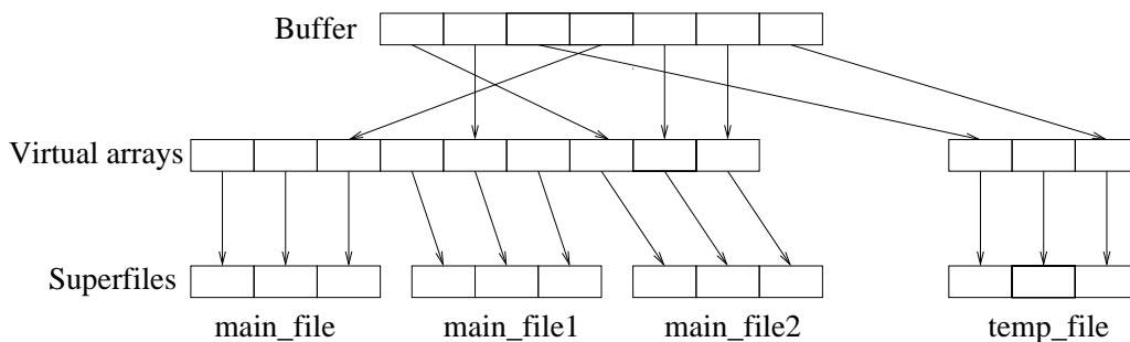
Figure 1.1: The buffer, virtual arrays, and files of the superfiles.
