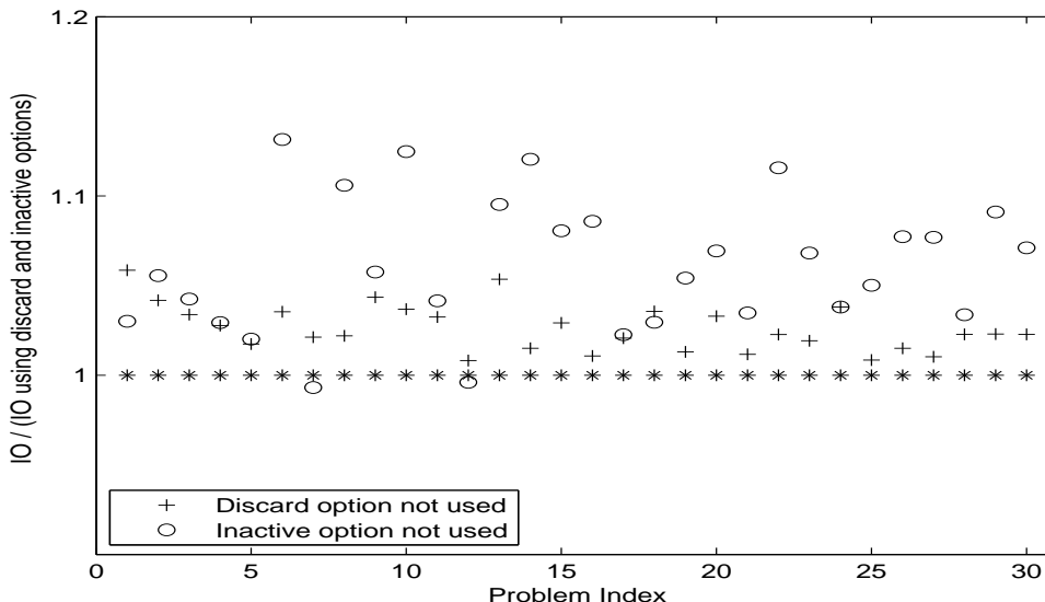
Figure 4.1: The ratios of the total number of input/output records within MA77_factor_solve with and without the discard and inactive options.
